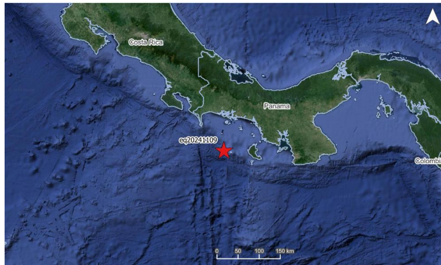
Figure 1 Information from the Earthquake Hazards Program of the United States Geological Survey regarding the earthquake event on 09 November 2024. Source: USGS 1
